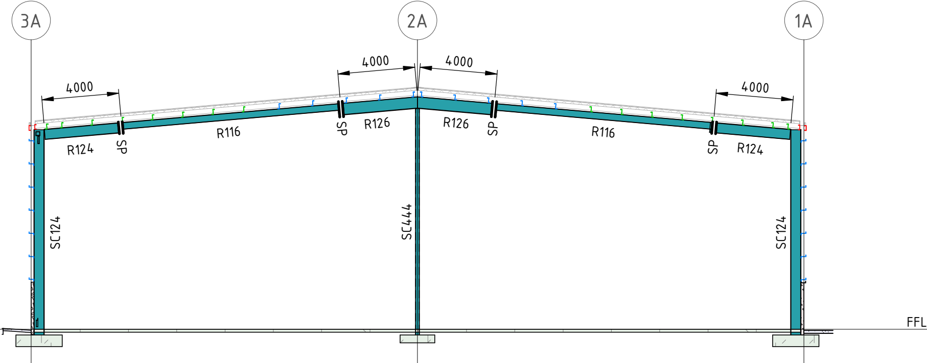
SECTION A4 SCALE 1 : 200
