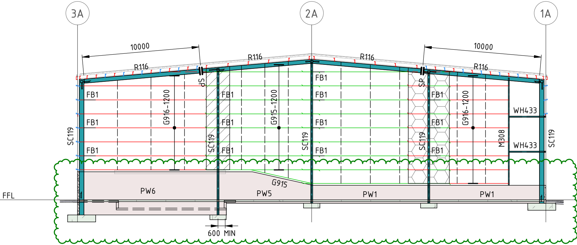
SECTION A1 SCALE 1 : 200
