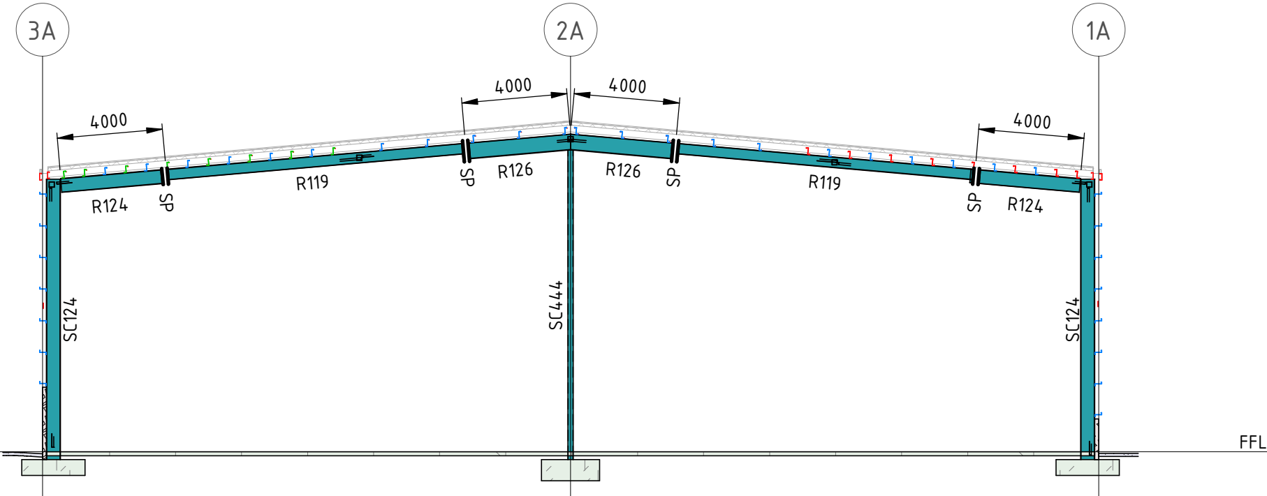
SECTION A2 SCALE 1 : 200
