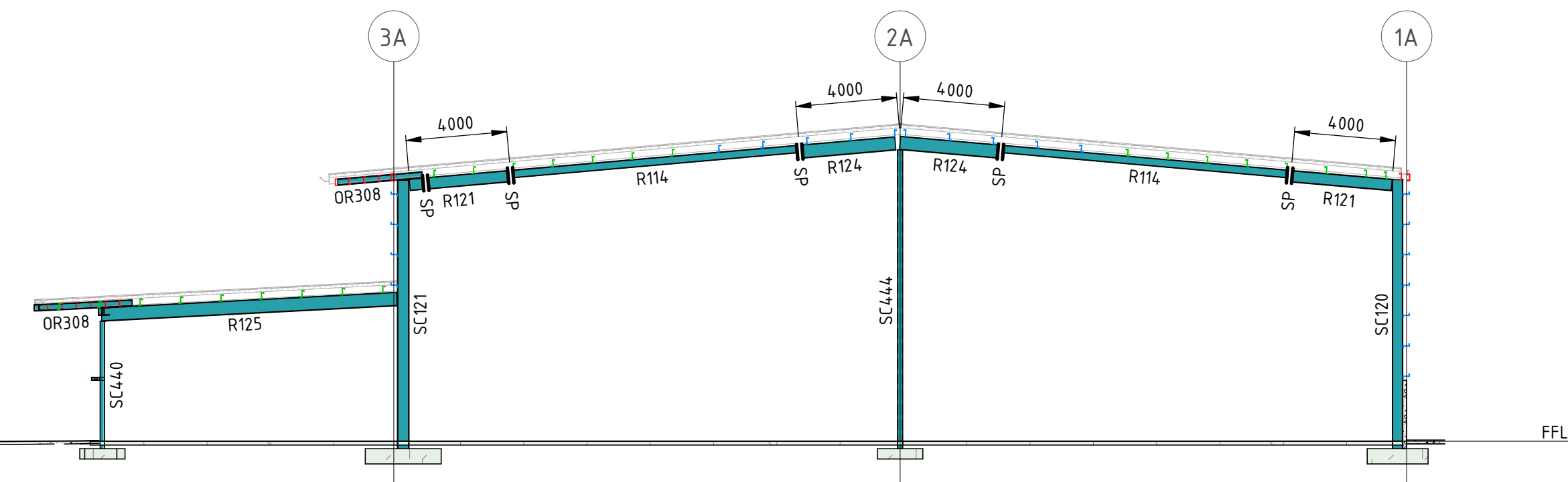
SECTION A8 SCALE 1 : 200
