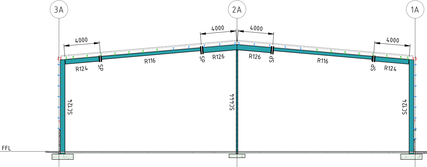
SECTION A3 SCALE 1 : 200
